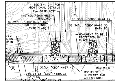
PATH IMPROVEMENTS NEAR SUNNYVALE WEST CHANNEL NO SCALE
