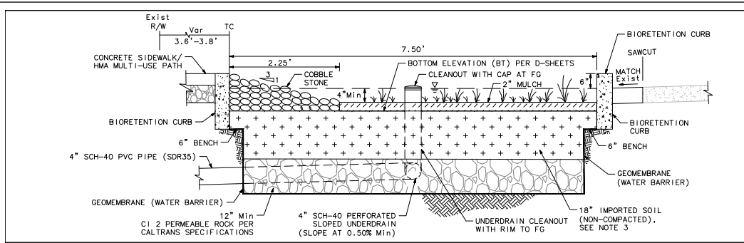
BIORETENTION DETAIL (TYPICAL) NO SCALE
